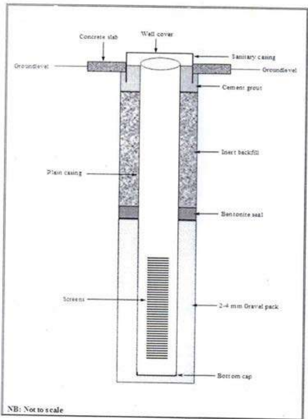
Schematic Design for Borehole Completion
